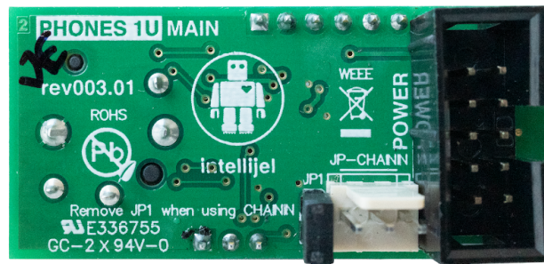
VERSION 2 has power, plus a 3-pin Link Connector (and normalizing jumper) on the rear panel
