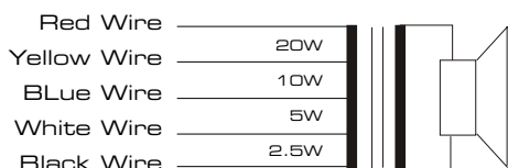
GB20/T Circuit diagram 100V Common
