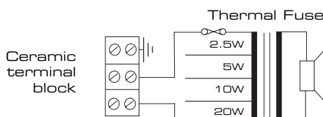
GB20/TC Circuit diagram 100V Common
