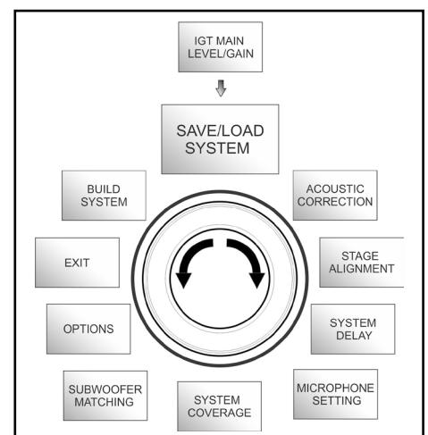
Menu Save/Load
