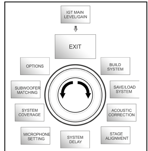
Exit Menu
